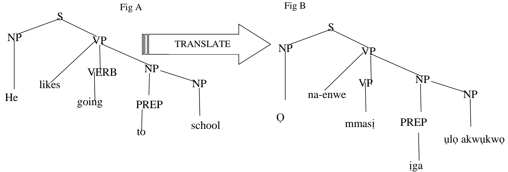
Figure 6 Syntax structure
