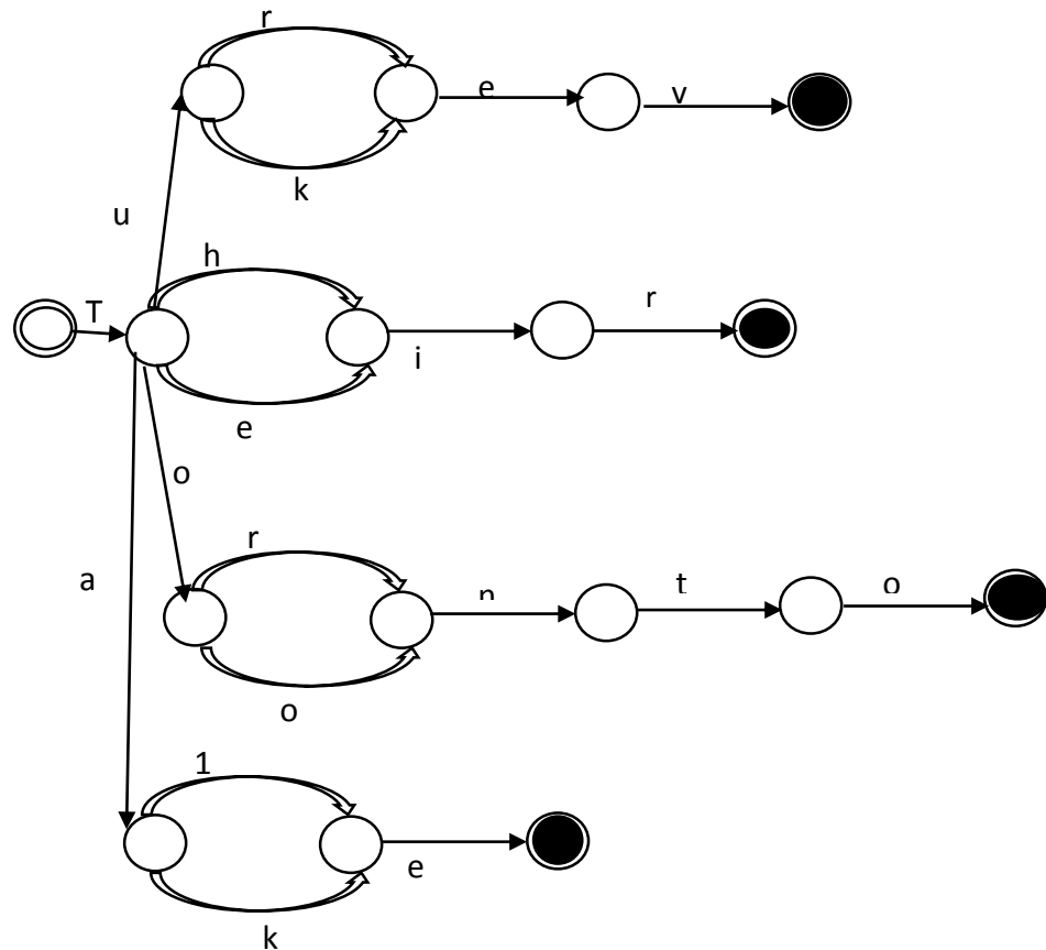
Figure 2: Finite State Automata to Identify English Language Token
