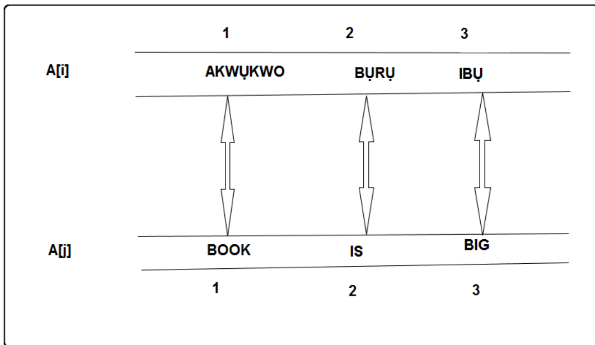
Figure 4 Word-based Mapping
