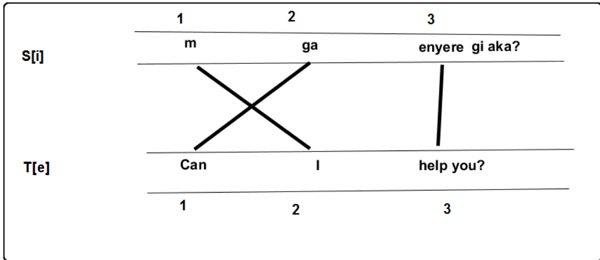
Figure 5 Phrase-based model
