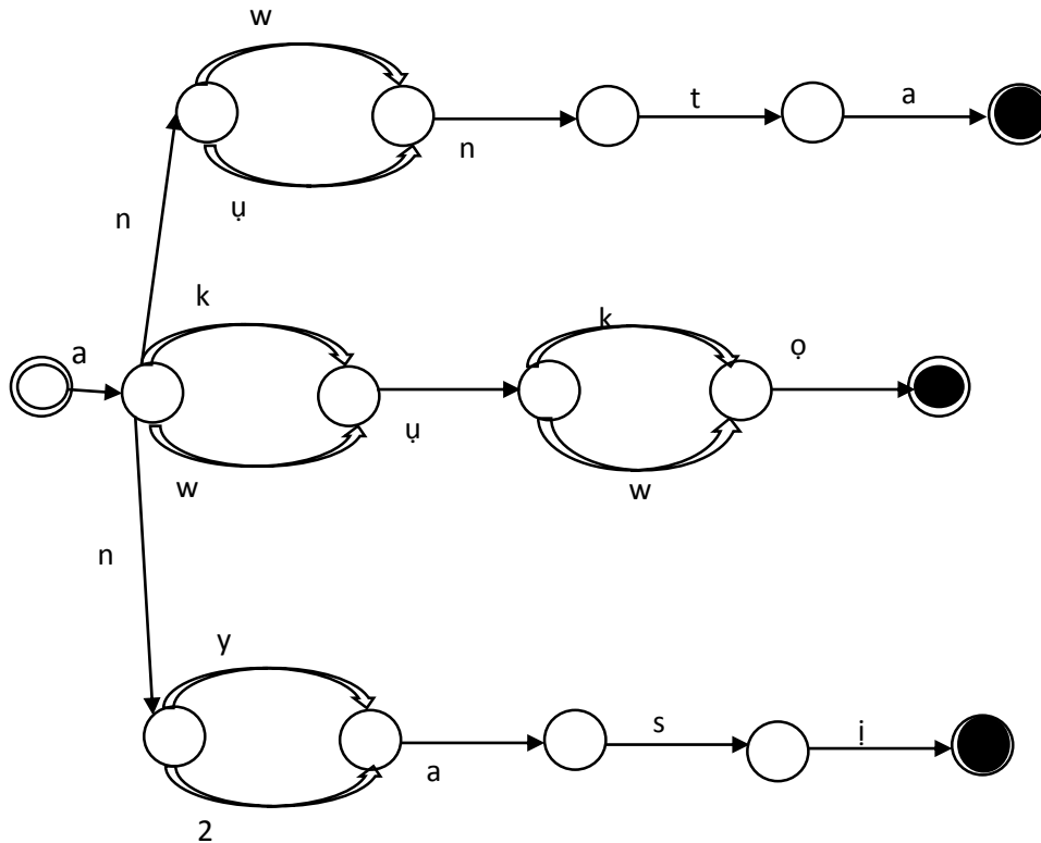
Figure 3 Finite State Automata to Identify Igbo Language Token
